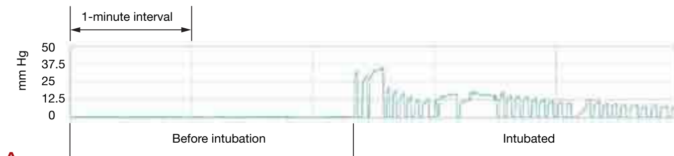
Figure 3 Capnography Waveforms
